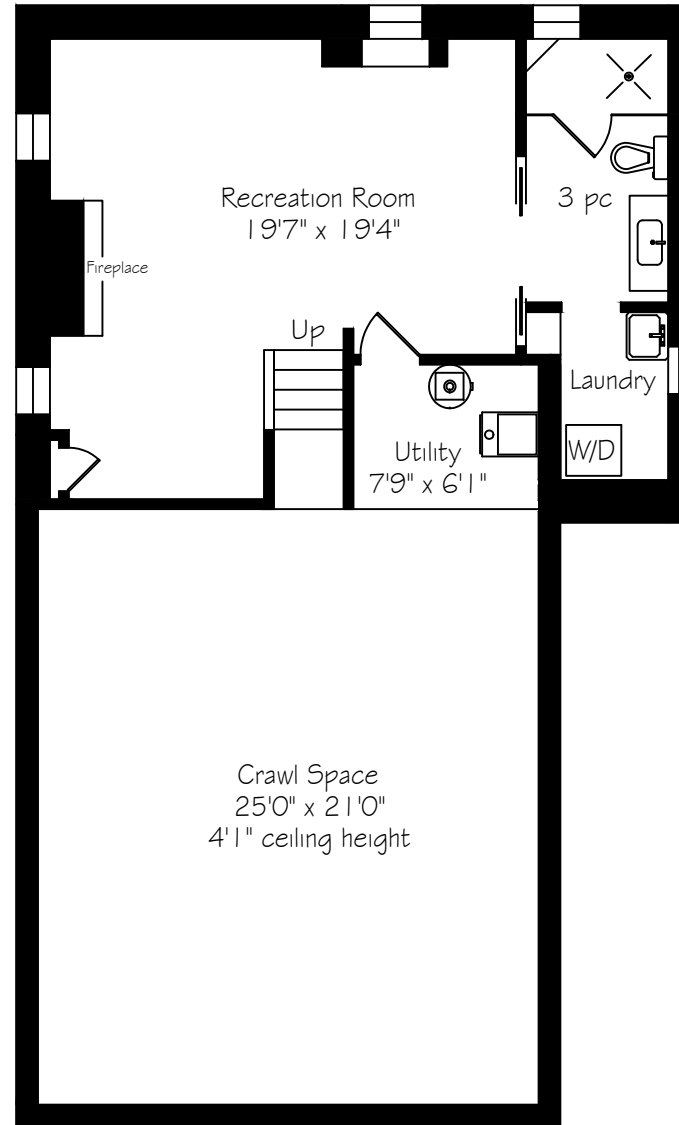
Lower Level 603 Square Feet + 590 Crawl Space
